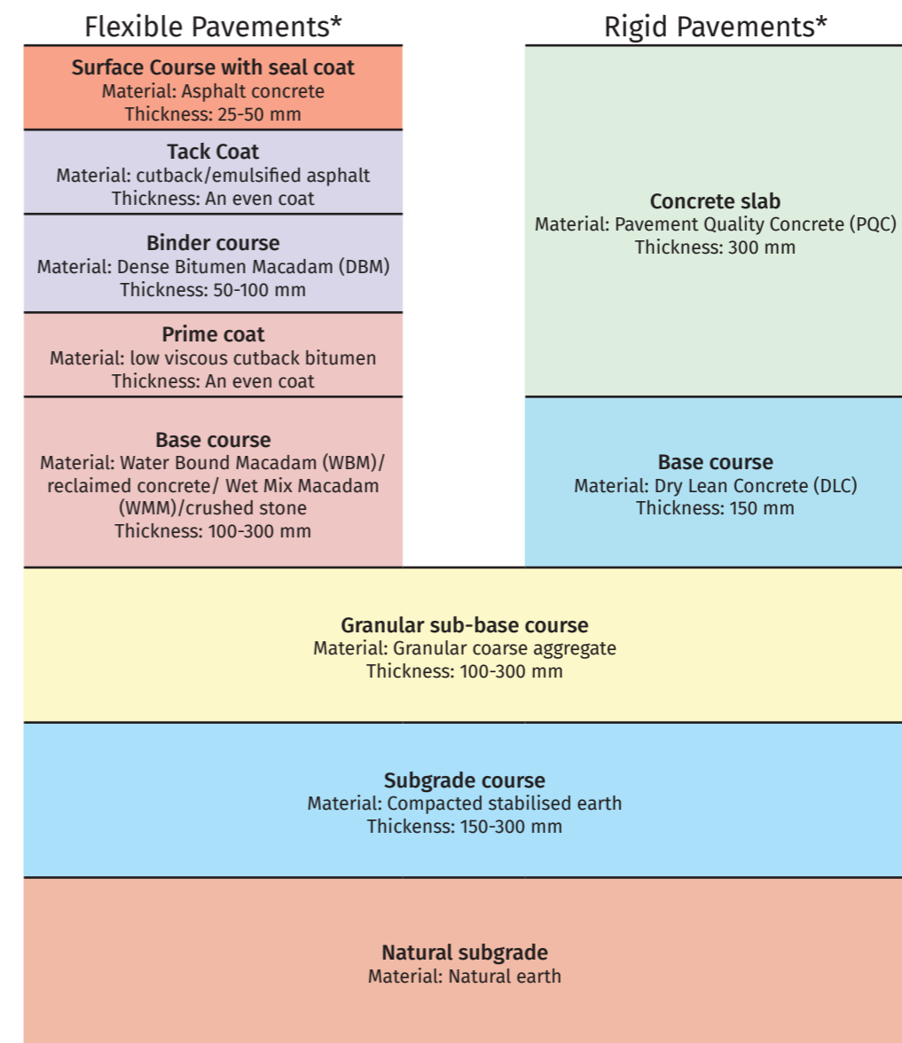
Fig. Layer composition of flexible and rigid pavements
